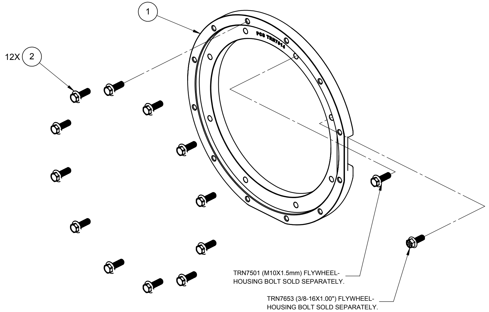
EXPLODE VIEW COMPONENTS SCALE: 1:4
