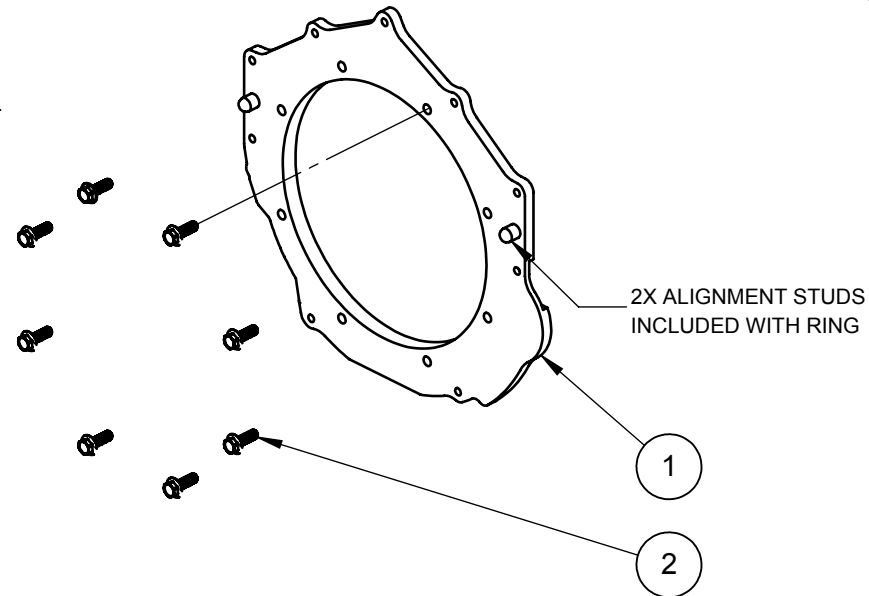
EXPLODED VIEW PARTS BREAKDOWN SCALE: 1:8
