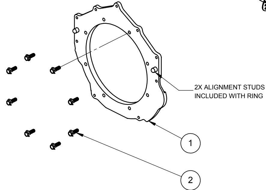
EXPLODED VIEW PARTS BREAKDOWN SCALE: 1:8
