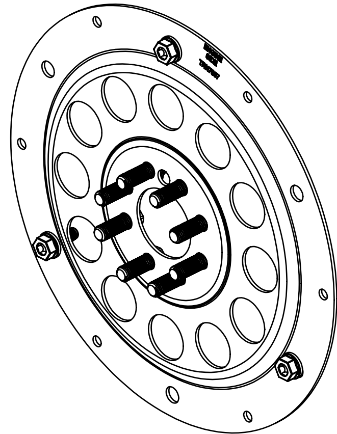
ISO VIEW ASSEMBLED SCALE: 3:8
